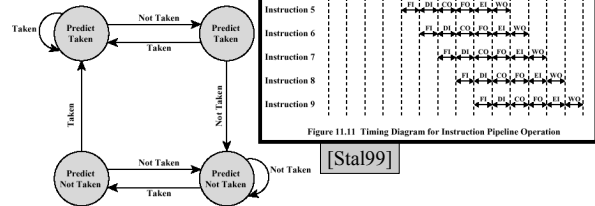
Figure 11.16 Branch Prediction State Diagram
