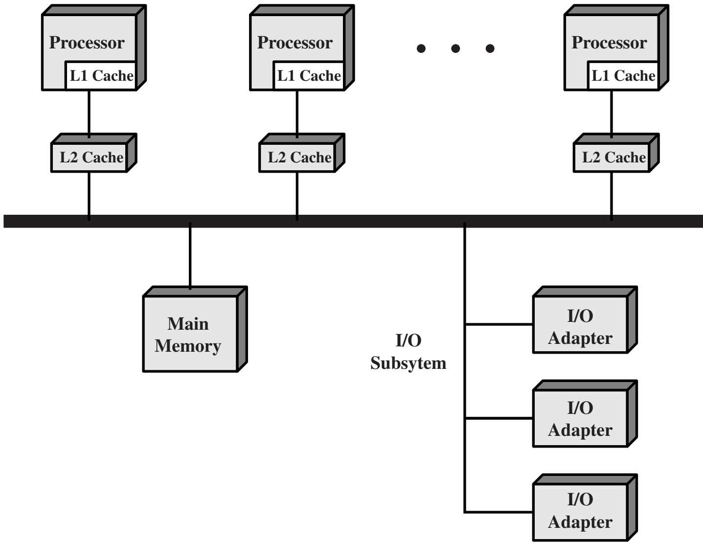
Figure 4.9 Symmetric Multiprocessor Organization
