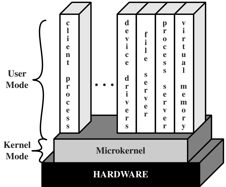
(b) Microkernel
