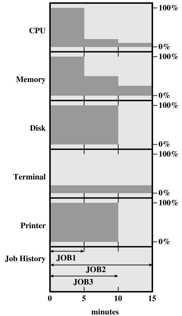
(b) Multiprogramming
