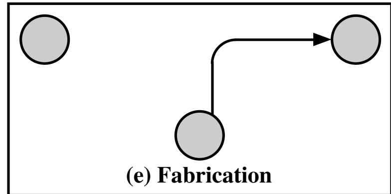
Figure 15.2 Security Threats
