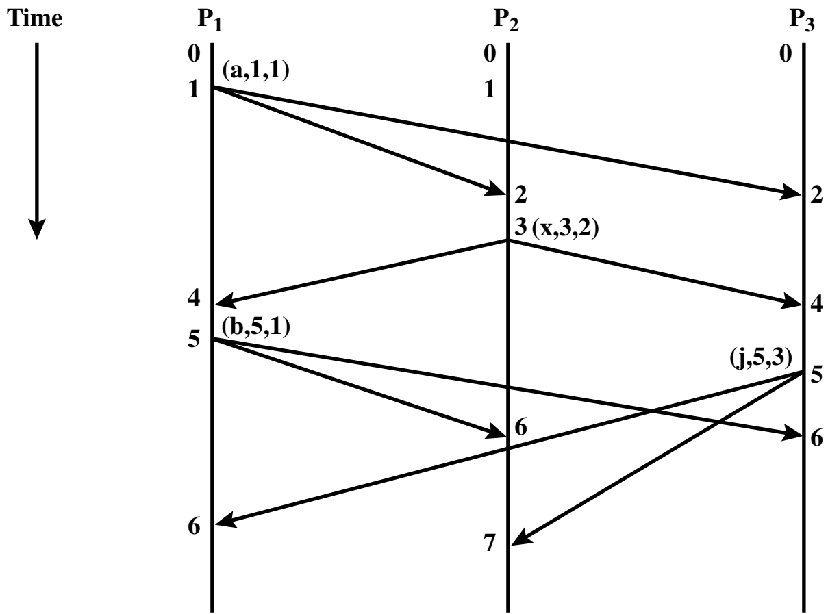
Figure 14.8 Example of Operation of Timestamping Algorithm
