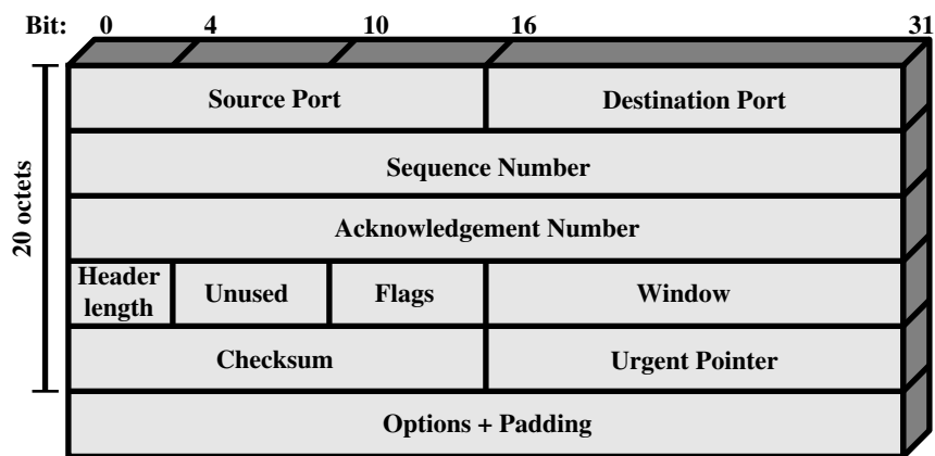
(a) TCP Header
