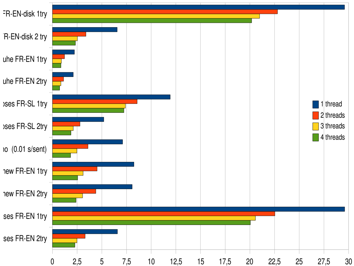
"Parlement europeen" threaded translation speed
