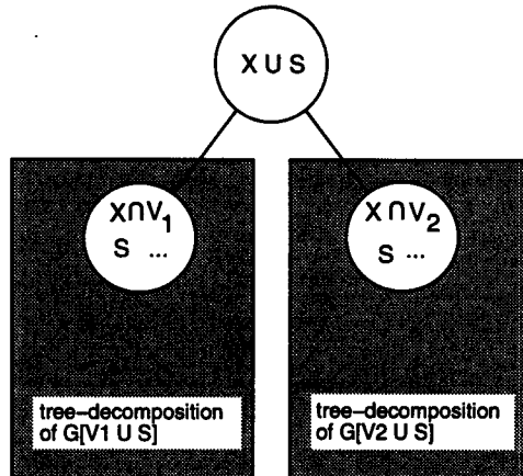
Figure 5: Illustration to approximation algorithm
