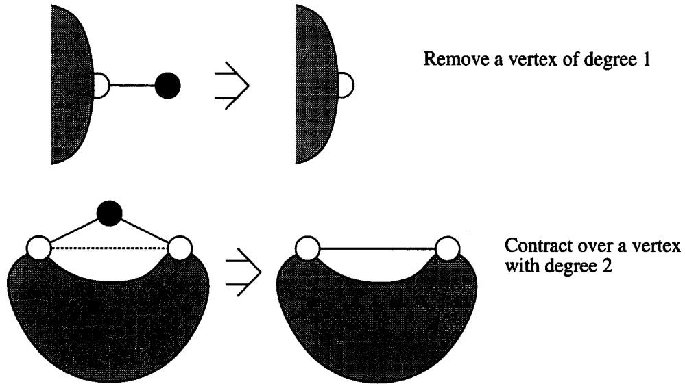
Figure 4: Rewriting a graph with treewidth \leq 2
